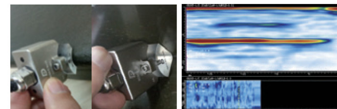
Aircraft CFRP Composite R Corner Inspection(Concave Probe)
