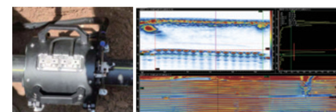
Inspection of PE electrofusion joint
