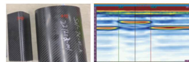
Ultrasonic detection of carbon fiber phased array for UAV arm
