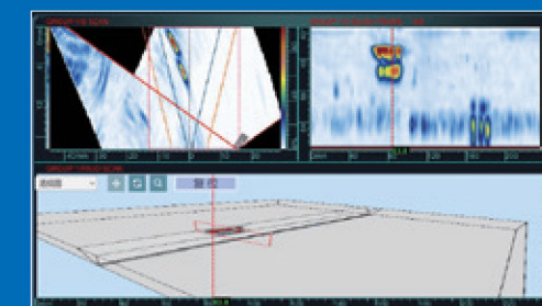
PA-3D Scanning
