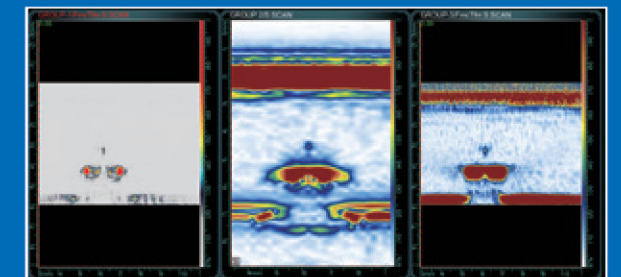
Copper, \phi 0.1\text{mm} flat bottom hole, FMC-PCI(left), PA(center), FMC-TFM(right)
