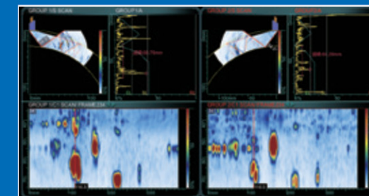
Pipeline longitudinal seam inspection
