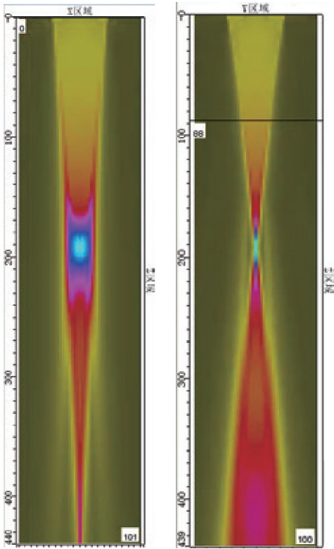
Simulation of sound field CIVA: underwater sound field in XZ and YZ respectively.
