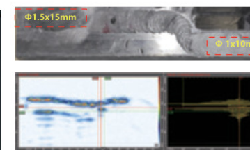
FSW friction stir welding inspection
